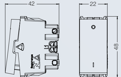
Interruptor bipolar simples
