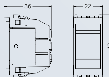
Interruptor persiana
