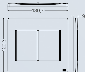
Placa Aro LED 4x4 6 POS
