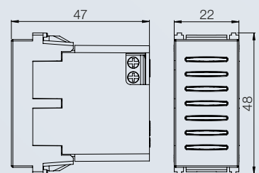
Campainha cigarra
