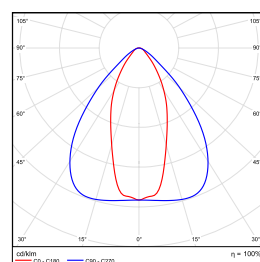
NARROW HIGH RACK
