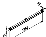
EM40006LED
