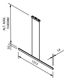
PD10150LED
