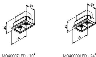
MO40007LED - 10°
