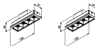
MO40008LED - 10°
