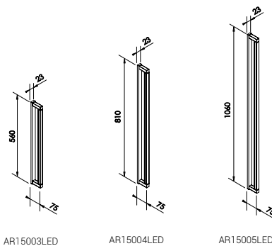
AR15003LED
