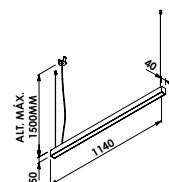
PD40001LED
